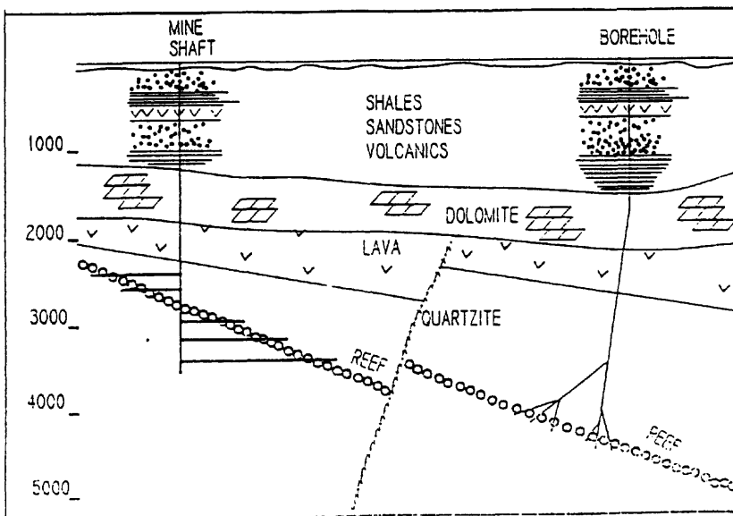
Figure 2. Typical mine Layout.
