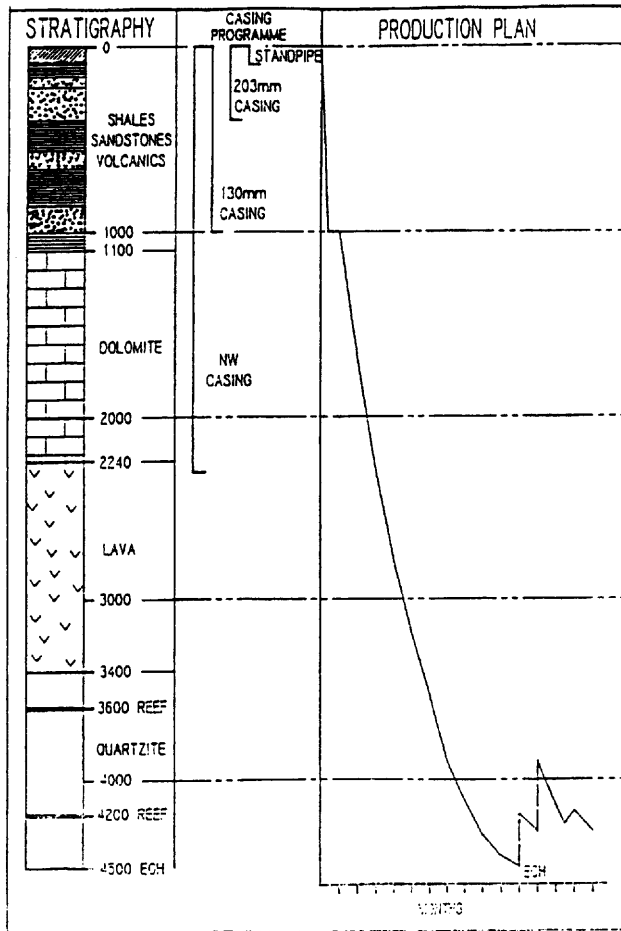
Figure 3. Typical Borehole Plan.
